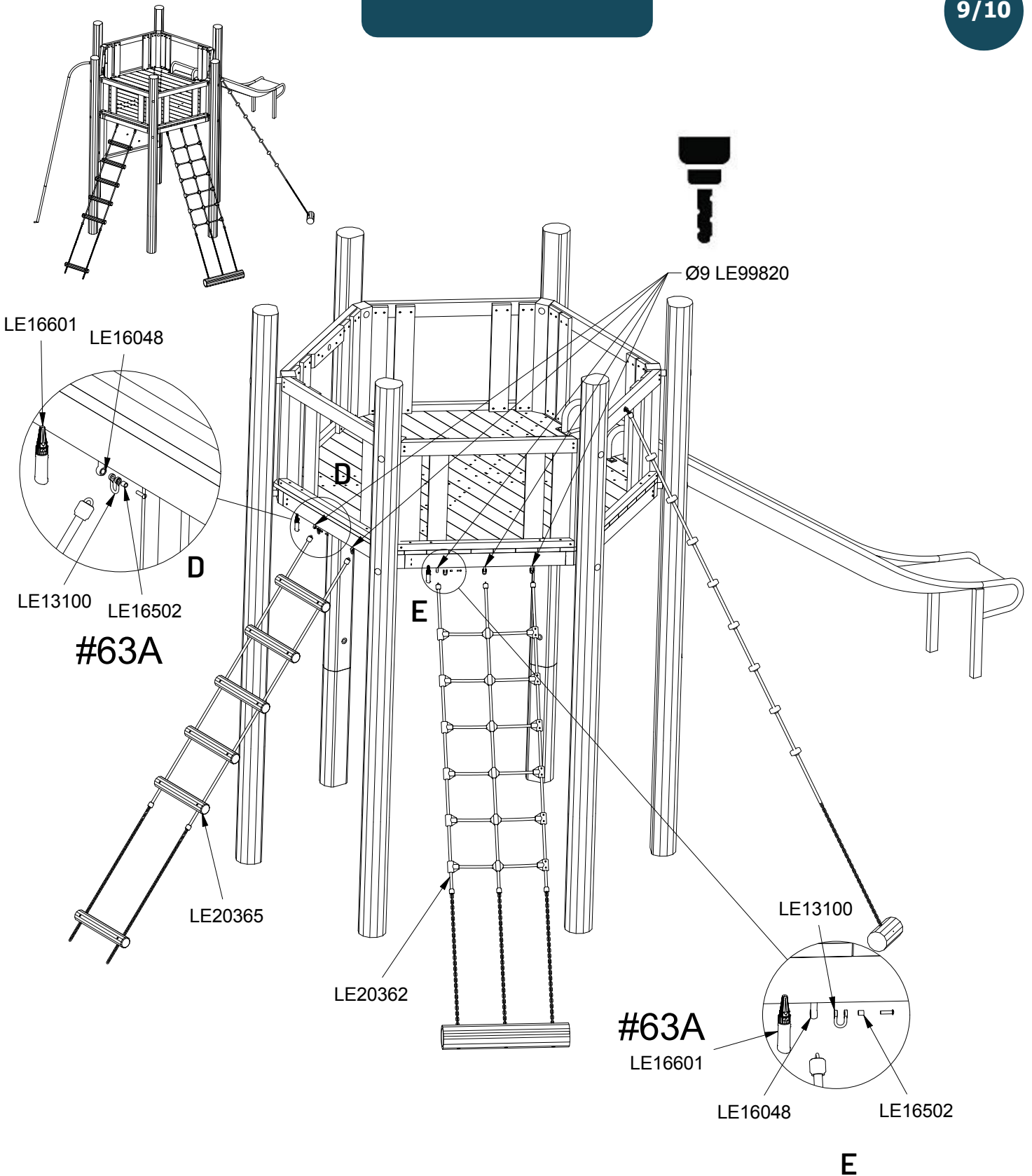
Parts List
